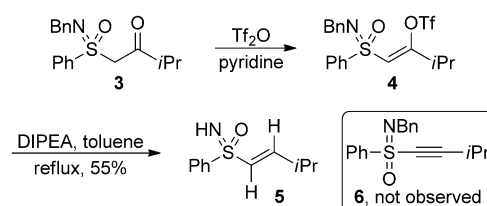
Scheme 2. Intramolecular redox reaction.
